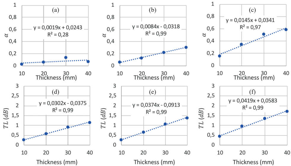
Figure 8: The average SACs and TLs of the homogenous luffa fiber samples with different thicknesses for low (a and d), medium (b and e) and high (c and f) frequency ranges (bulk density: 73.6 \text{ kg/m}^3 ).
