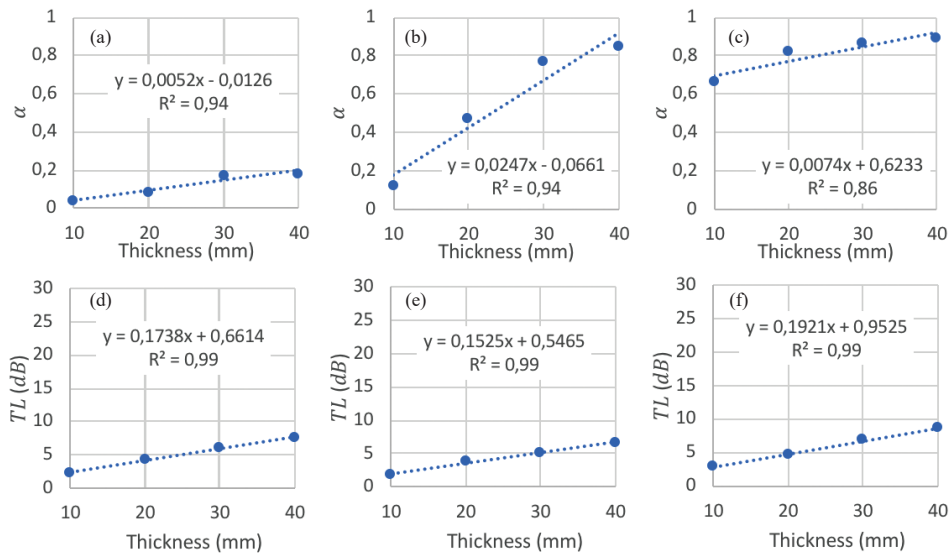
Figure 12: The average SACs and TLs of the hybrid LJL samples with different thicknesses for low (a and d), medium (b and e) and high (c and f) frequency ranges (bulk density: 178.0 kg/m 3 ).
