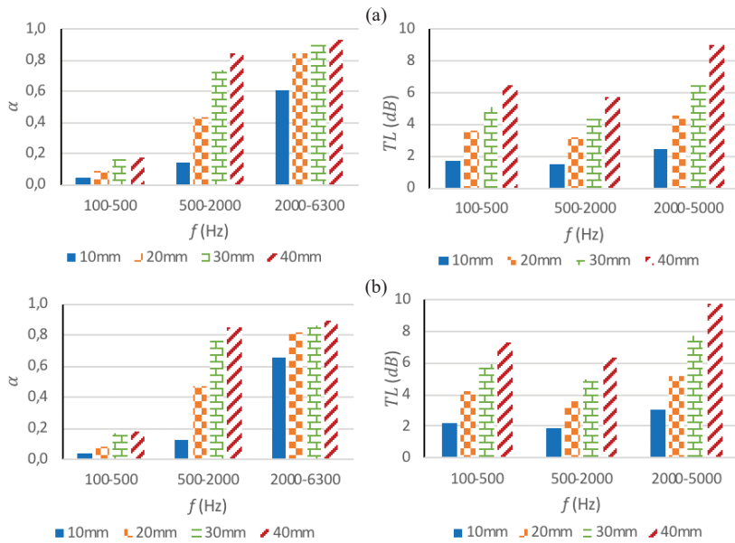
Figure 10: The SACs (left) and TLs (right) of the hybrid (a) JLJ and (b) LJJ samples with different thicknesses for different frequency ranges.
