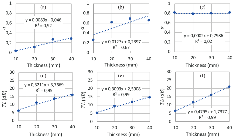
Figure 7: The average SACs and TLs of the homogenous jute fiber samples with different thicknesses for low (a and d), medium (b and e) and high (c and f) frequency ranges (bulk density: 419.8 kg/m 3 ).
