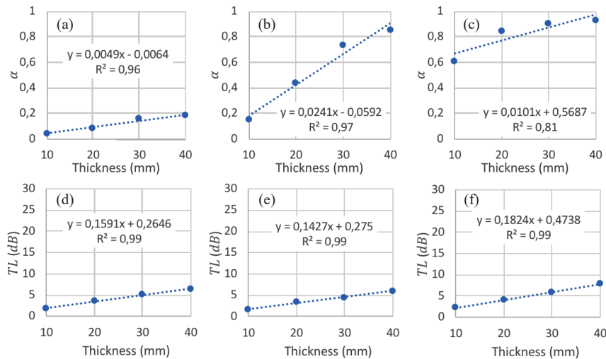
Figure 11: The average SACs and TLs of the hybrid JLJ samples with different thicknesses for low (a and d), medium (b and e) and high (c and f) frequency ranges (bulk density: 187.4 kg/m 3 ).
