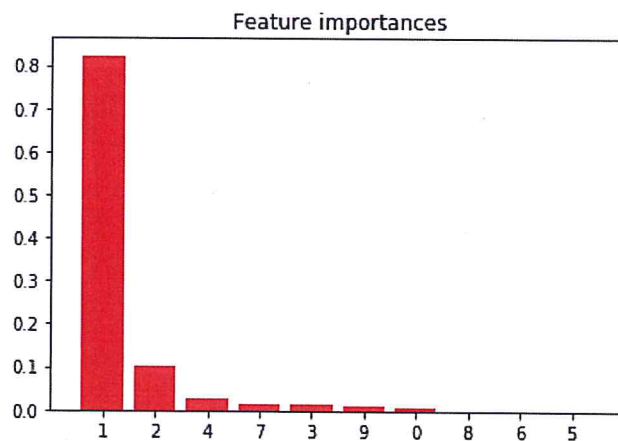
Figure 9 : Feature importance for max_depth=5
