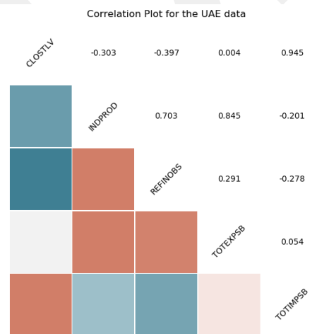
Figure 3. Correlation plots for Russia, USA and UAE
