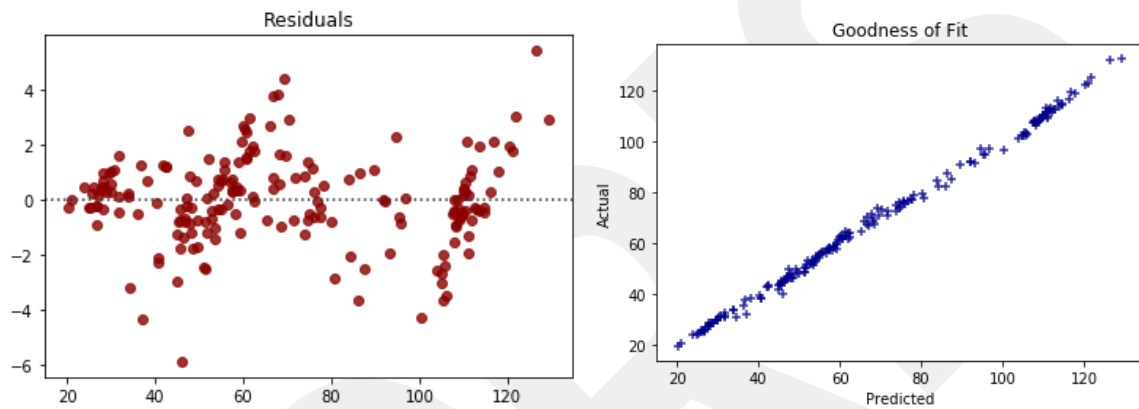
Figure 8. Residuals and Goodness of Fit graphs for train sample
