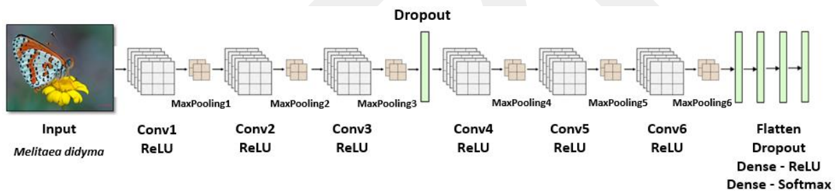
Figure 8: Convolutional neural network (CNN) model used for butterfly classification
