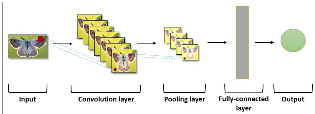
Figure 5: Convolutional neural network architecture
