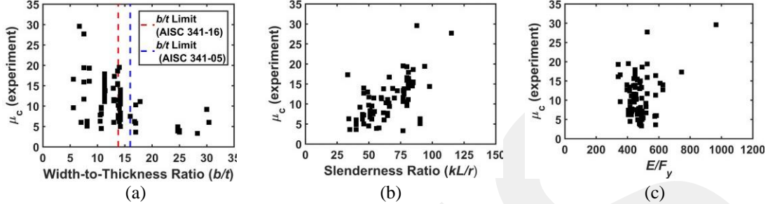
Figure 3. Ductility capacity of the collected 79 specimens at fracture: (a) interaction between ductility capacity at fracture ( \mu_c ) and width-to-thickness ratio ( b/t ), (b) interaction between \mu_c and slenderness ratio ( KL/r ), and (c) interaction between \mu_c with the mechanical properties ( E/F_y ).
