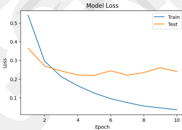
Figure 3.13 BERTweet loss function curve
