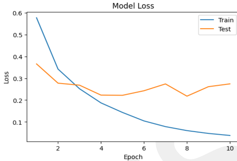
Figure 3.10 RoBERTa loss function curve
