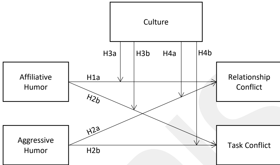
Figure 1. Research model 1.
