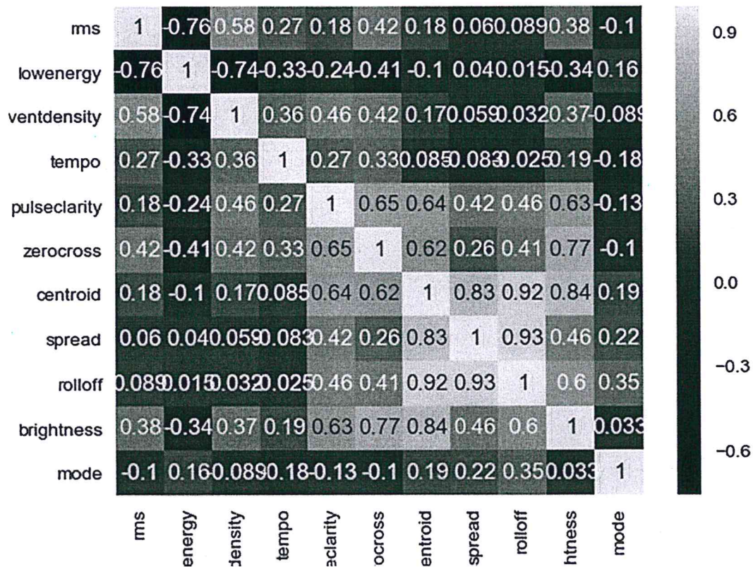
Figure 10: Correlation Coefficient
