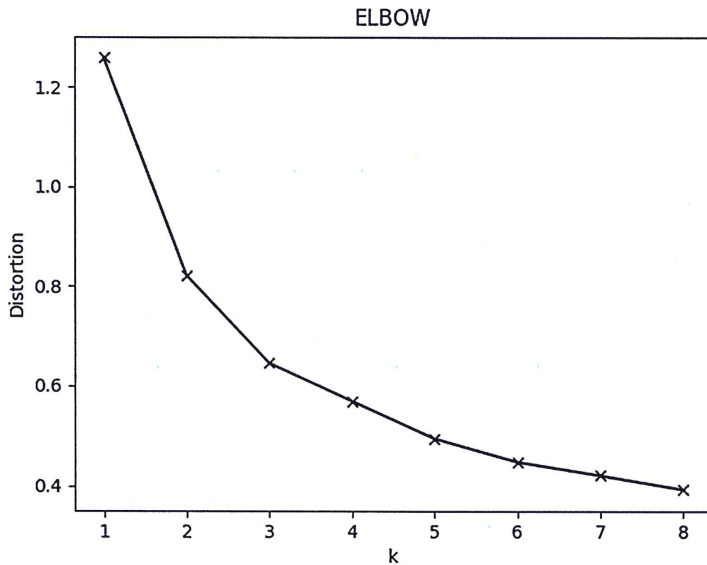
Figure 5: Elbow Method
