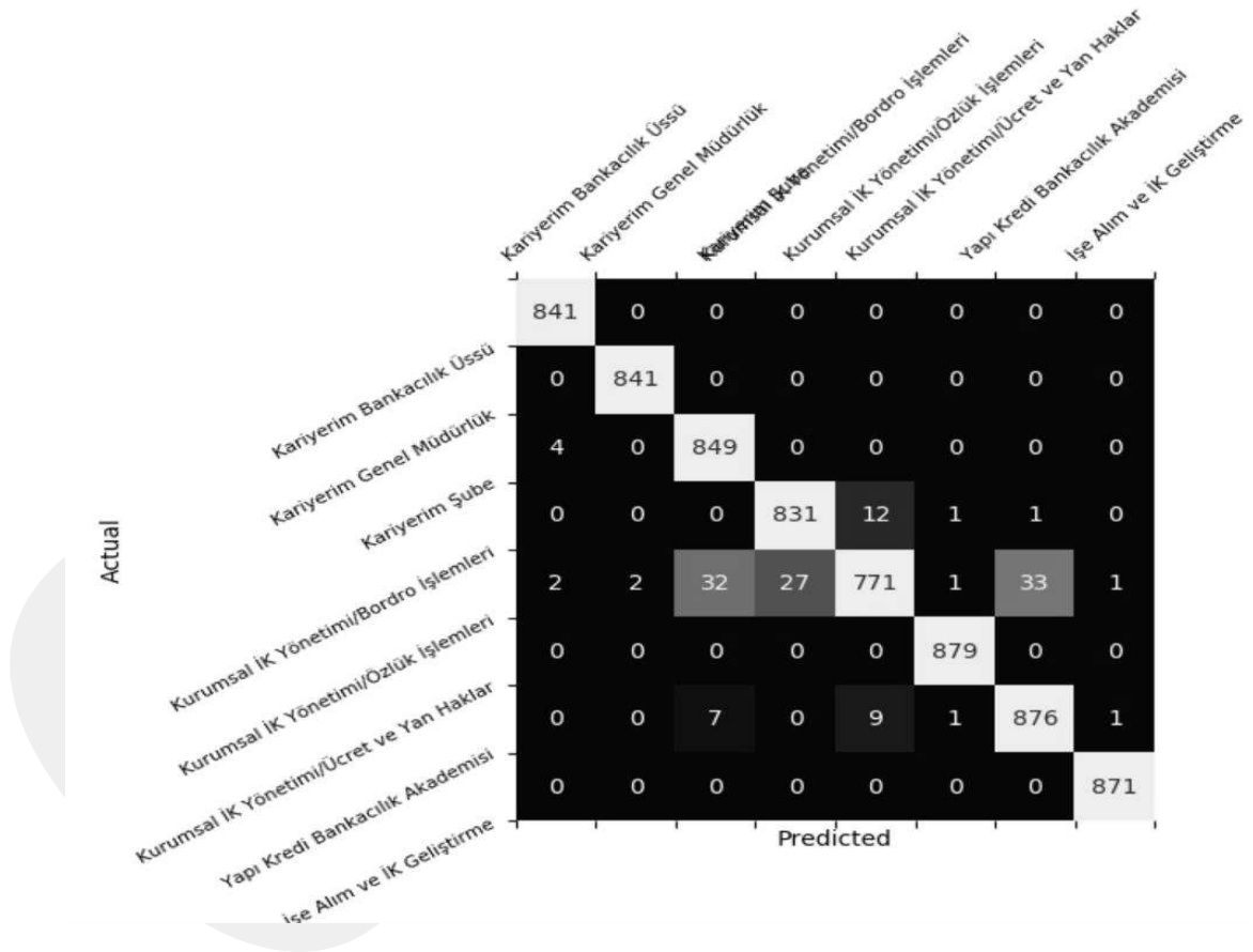
Figure 7: Confusion Matrix of Multinomial Naive Bayes with Grid Search
