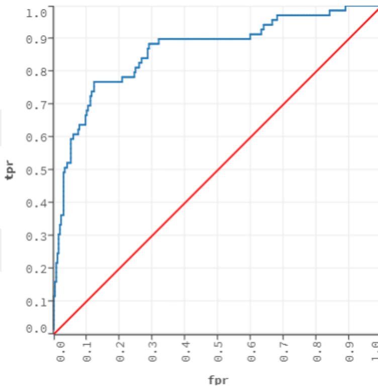
Figure 12 - DNN Validation AUC
