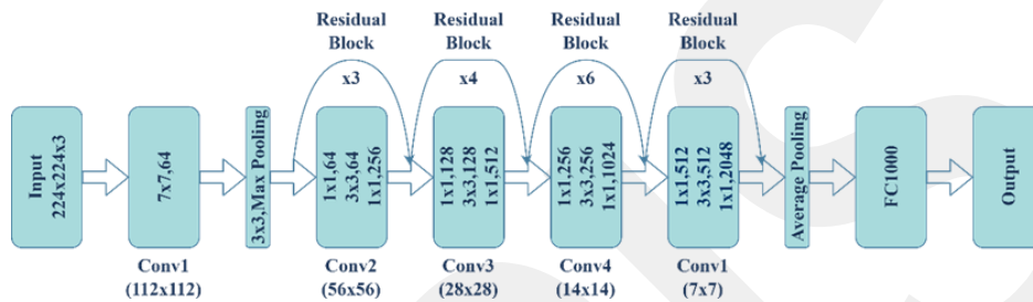
Figure 3. ResNet50 Architecture
