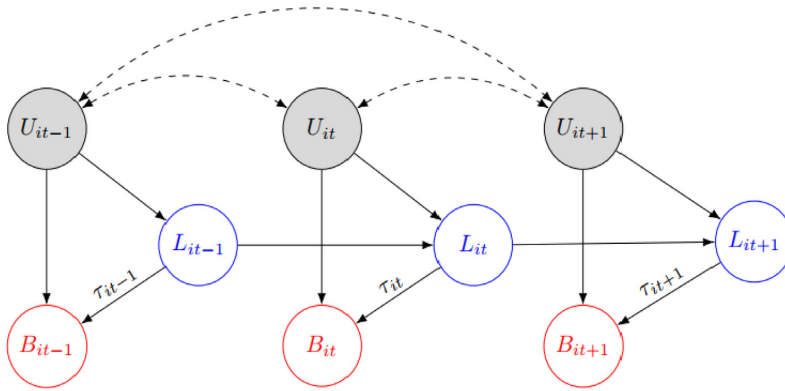
Figure 2. DAG \mathcal{G}_1 .
