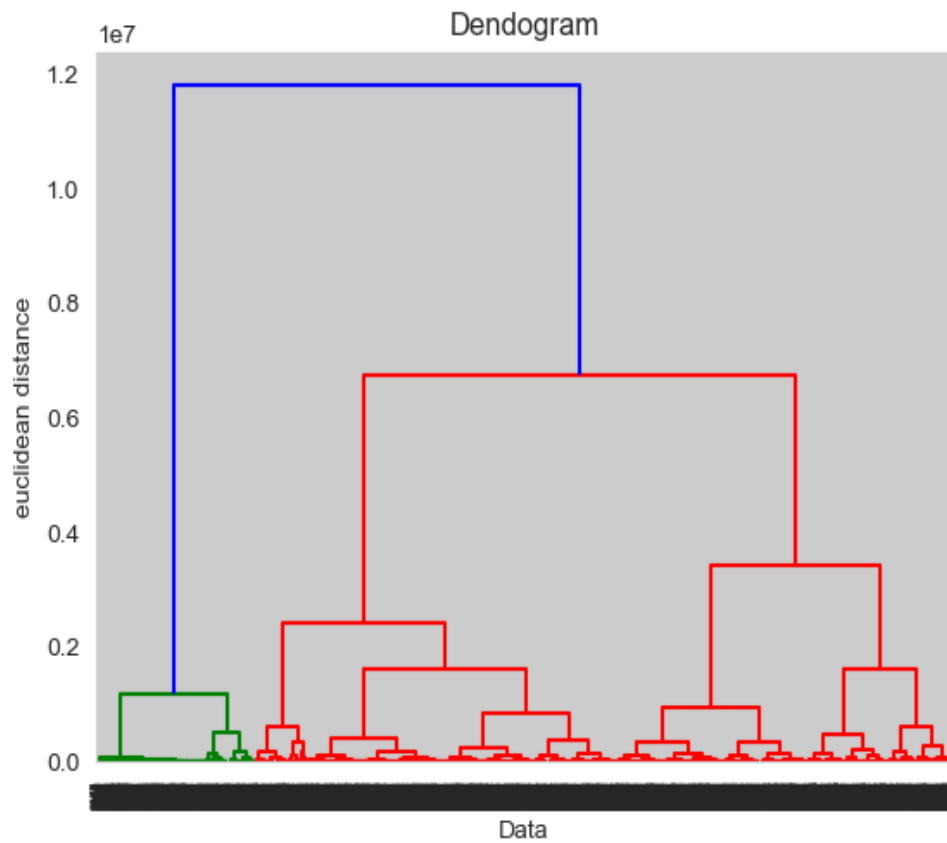
Figure 6. Euclidean Distance
