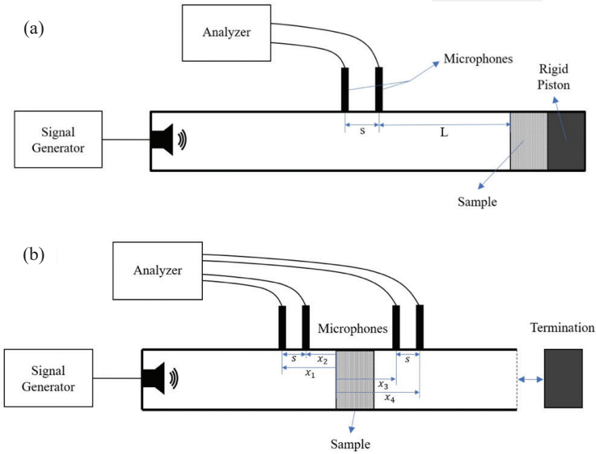
Figure 2: The schematic pictures of the experimental setups for the SAC (a) and TL (b) measurements.
