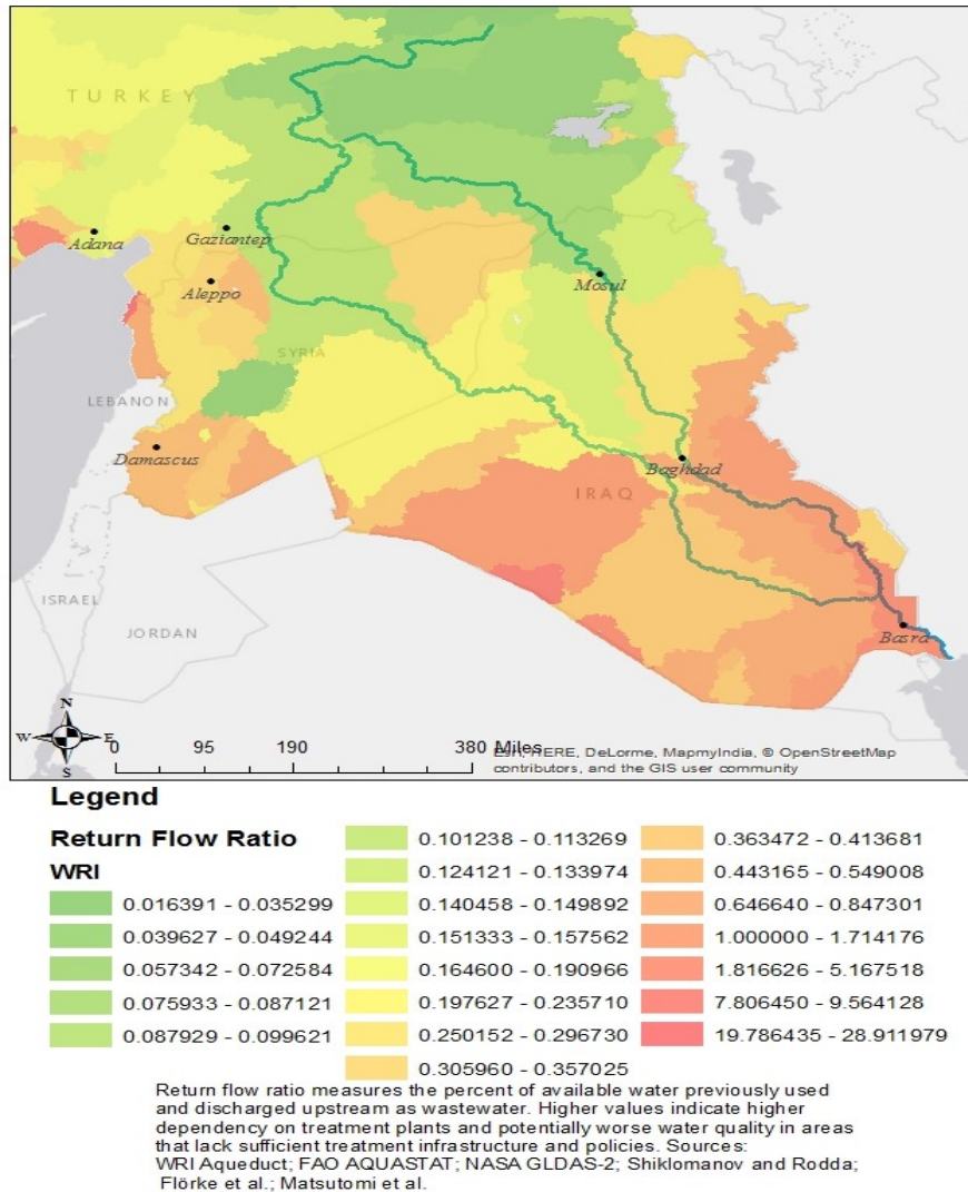
Figure 11.9. Return Flow Ratio
