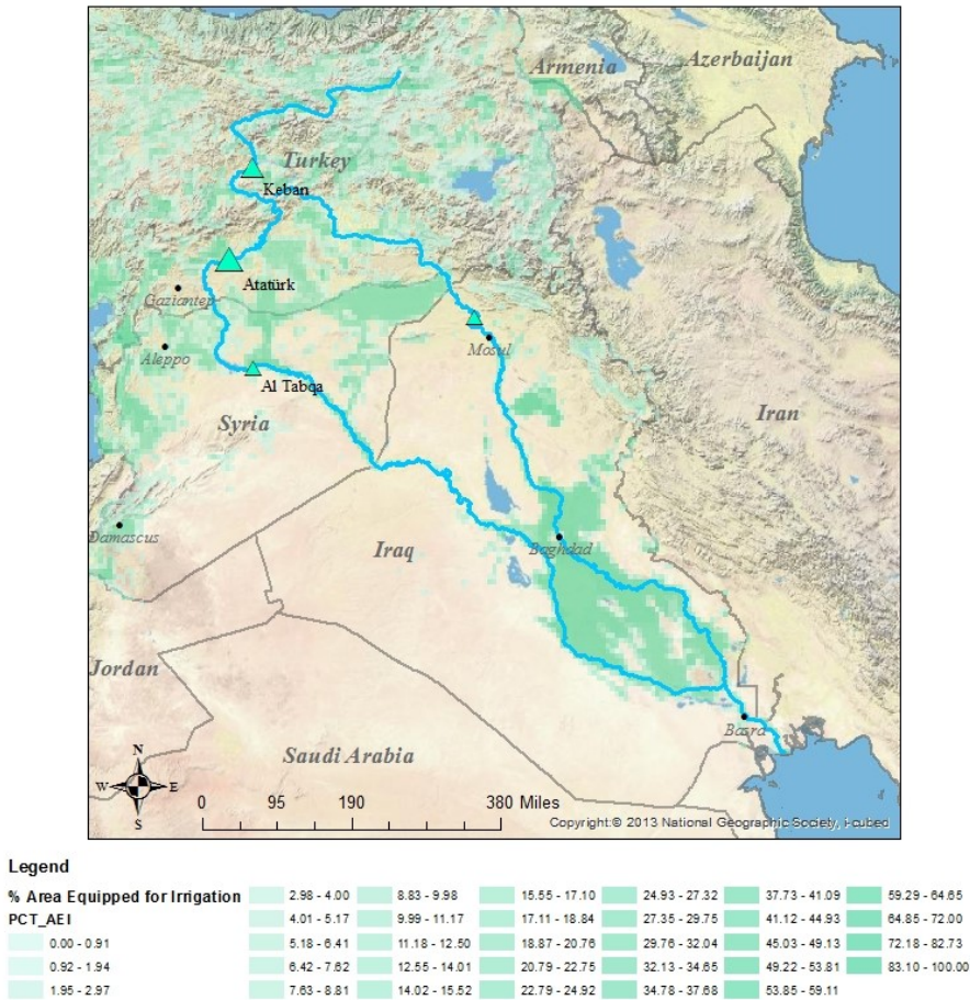
Figure 11.7. Irrigated Lands in the Euphrates-Tigris Basin
