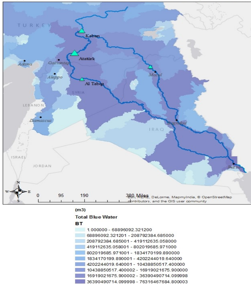
Figure 11.5. Total Blue Water in Cubic Meters
